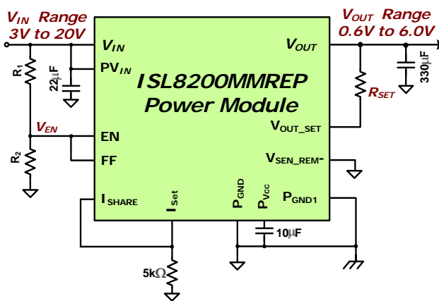
FIGURE 1. COMPLETE 10A DESIGN, JUST SELECT R_{SET} FOR THE DESIRED V_{OUT}
